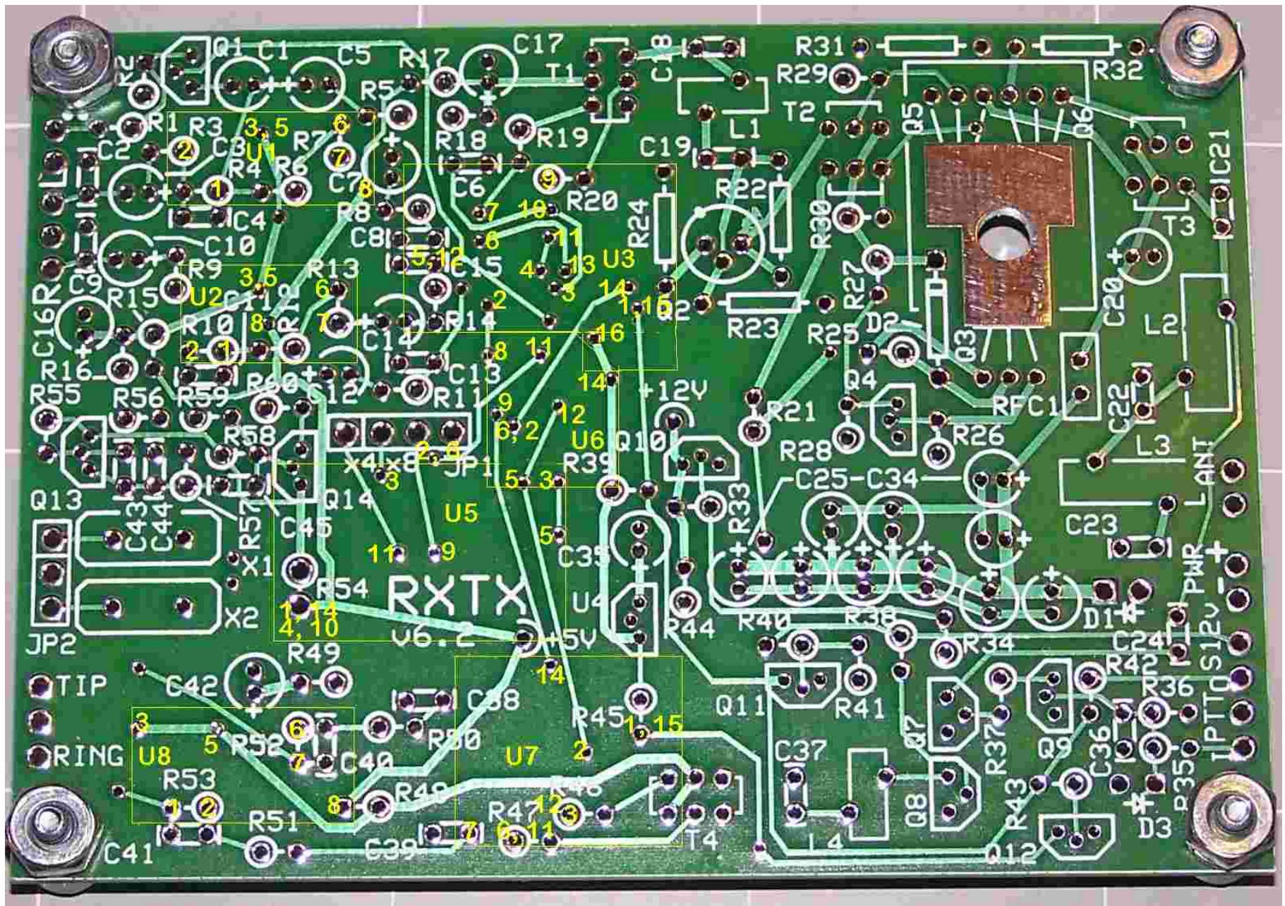
Top of Board, Annotated with IC Pinout test points.
