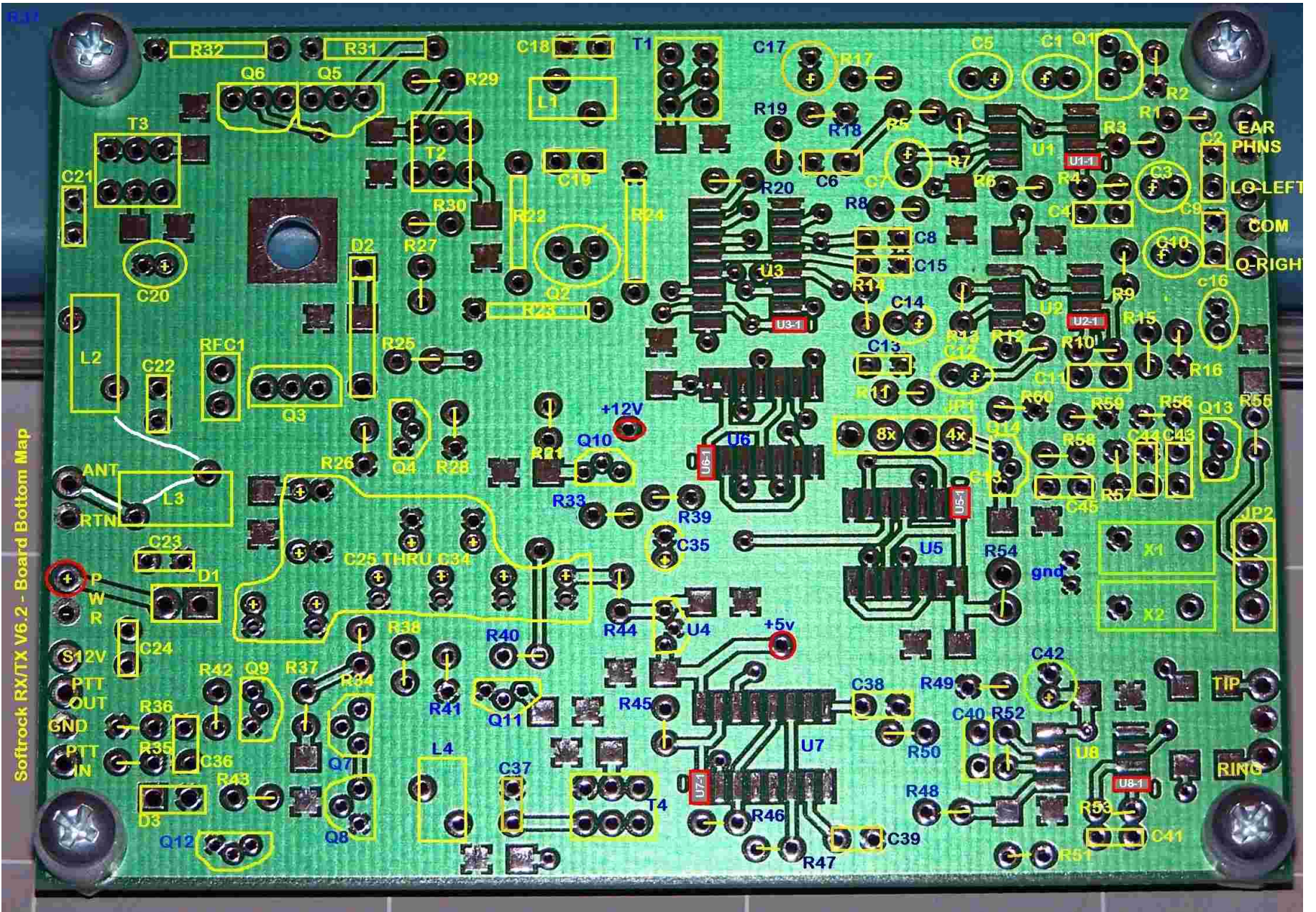
Bottom of Board, Annotated with Components from Top Silkscreen
